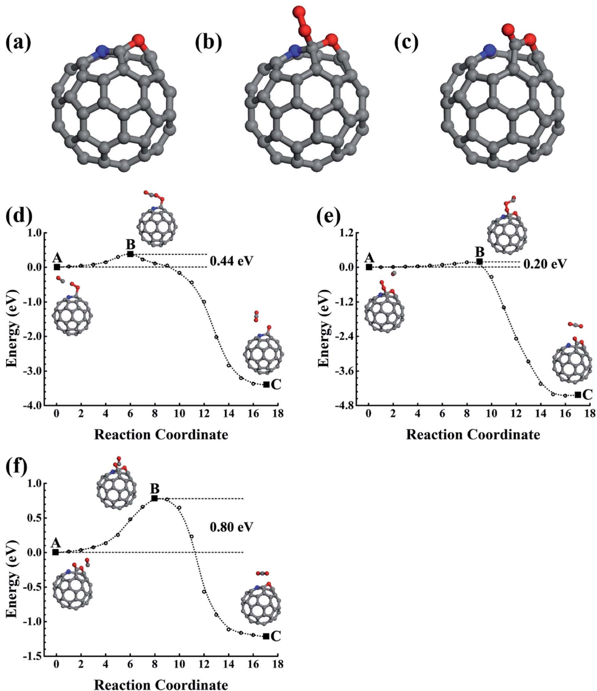
Fig. 3 (a) Structural skeleton illustrations for the C_{59}NO oxide; and (b) the lowest energy structure of O_2 molecules on the C_{59}NO oxide. (c) The structure of C_{59}NO_2 . (d)–(f) The optimized reaction paths for CO oxidation on C_{59}N and its oxides catalysts. The initial, final, saddle, and meta-stable intermediate states are illustrated in the inset images. C, N, and O are represented by the grey, blue, and red balls.
