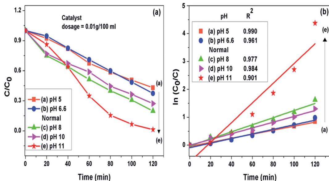
Fig. 8 (a) Comparison of photocatalytic activity of g-C_3N_4 at different pH condition (b) \ln(C_0/C(t)) for MB degradation with g-C_3N_4 at different pH condition as a function of simulated solar irradiation time.
