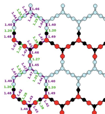
Fig. 2 Calculated bond length for the monolayers A, B, C and D shown in Fig. 1. The bond lengths illustrated repeat themselves periodically along the zigzag direction.
