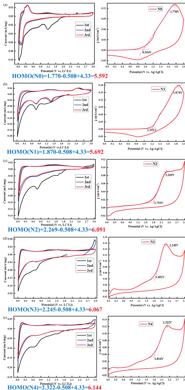
Fig. 5 (a–e) Cyclic voltammograms (CVs) of NG- \text{N}_{0-4} anode in LIB as a function of attached groups, and comparison of oxidation energy HOMO values with the cyclic voltammograms of the nanographenes in acetonitrile using tetrabutylammonium perchloride as electrolyte.
