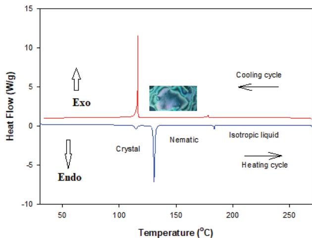
Fig. 2 DSC thermogram for I upon second heating/cooling cycles with heating rate 10\text{ °C min}^{-1} .
