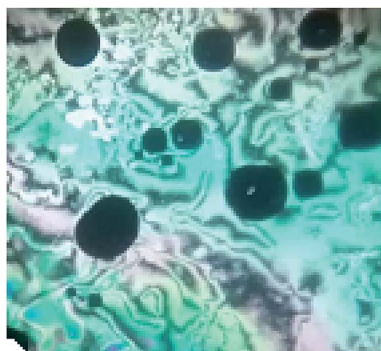
Fig. 4 Nematic mesophase texture under a polarized optical microscope for supramolecular complex IB at 126\text{ °C} upon heating.
