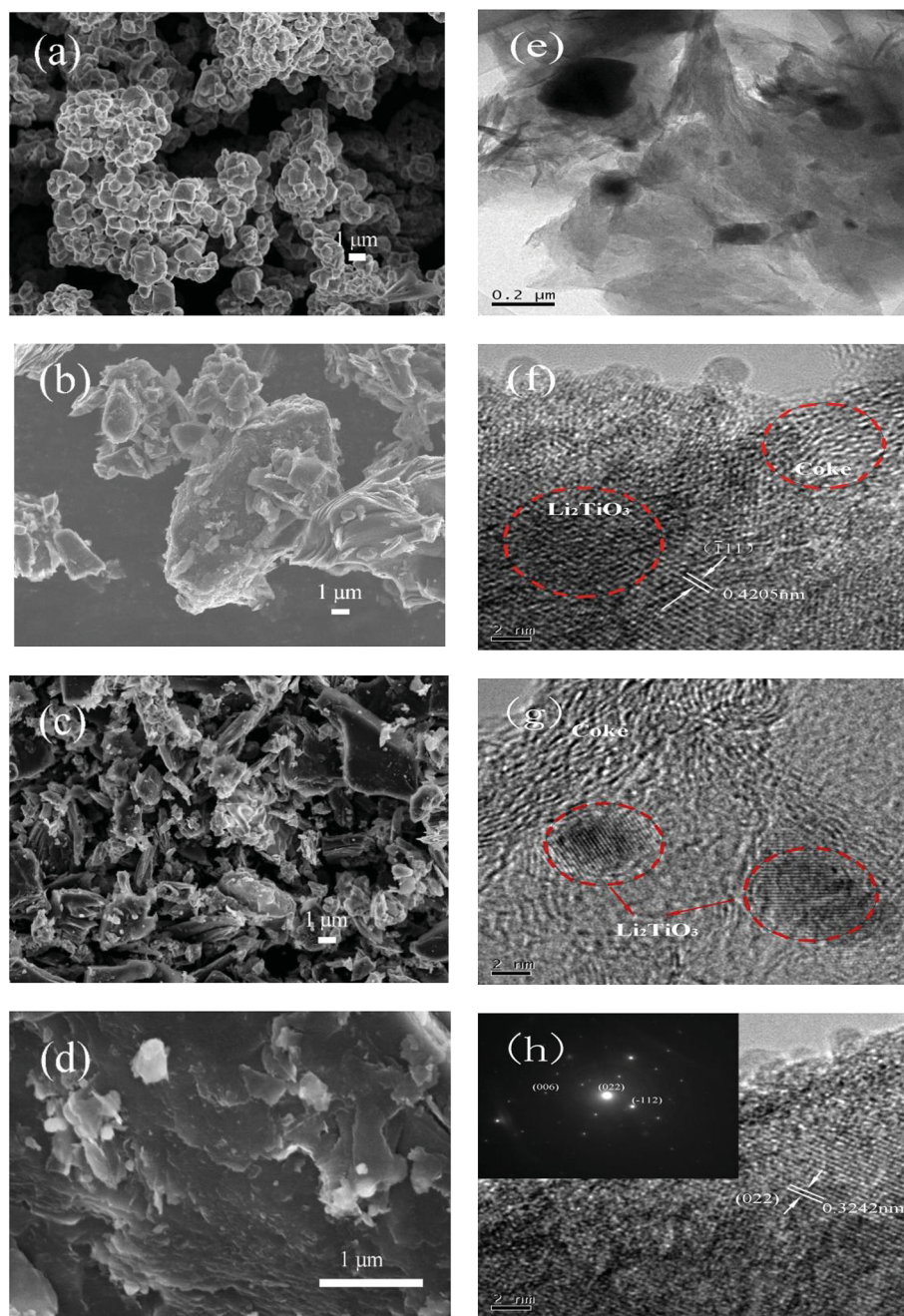
Fig. 2 SEM images of \text{Li}_2\text{TiO}_3 (a), petroleum coke (b), and LTOC with different resolutions (c) and (d). TEM of LTOC (e), (f), (g), and (h).
