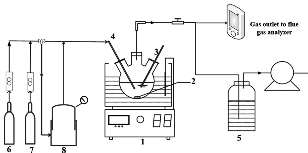
Fig. 1 Experimental apparatus for Fe(III)EDTA reduction by ascorbic acid ((1) heat collection-constant temperature type magnetic stirrer; (2) magnetic stirrer; (3) the pH electrode; (4) inlet for nitrogen or a mixture of NO and N_2 ; (5) buffer tank; (6) N_2 cylinder; (7) NO cylinder; and (8) cylinder containing a mixture of NO and N_2 ).
