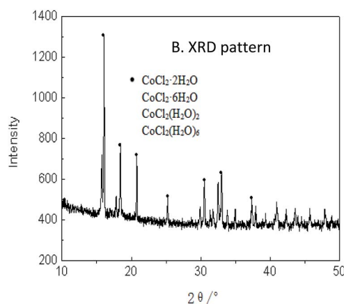
Fig. 5 Photograph (A) and XRD pattern (B) of products of \text{CoCl}_2 and its crystal water obtained by extraction.
