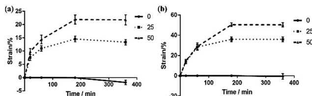
Fig. 4 Dynamic response curves of dual-responsive ONHs at (a) 32 °C and (b) 70 °C.
