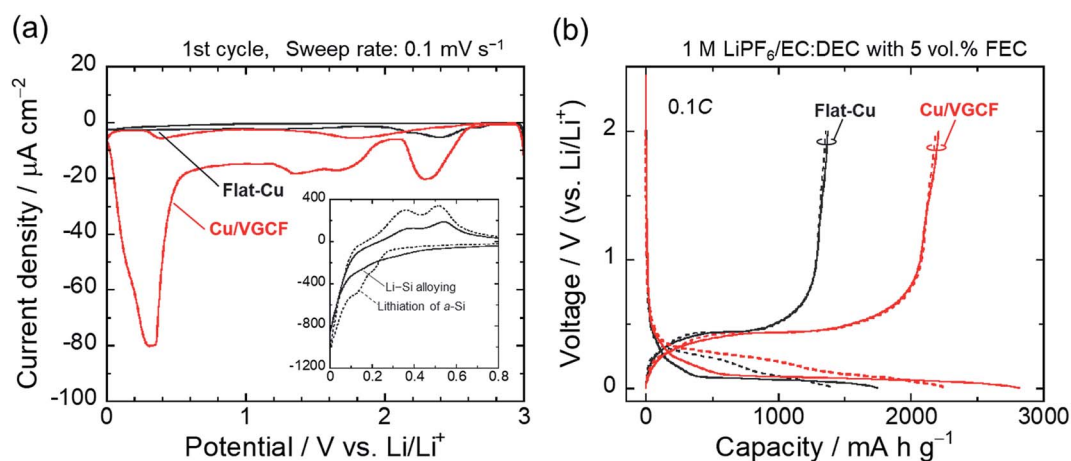
Fig. 4 (a) Cyclic voltammograms of Cu/VGCF and flat-Cu substrates in 1 M \text{LiPF}_6/\text{EC}:\text{DEC} (50 : 50 vol%) with 5 vol% FEC in the potential range of 0.0–3.0 V vs. Li/Li + . (b) Initial charge–discharge properties of Si electrodes prepared using commercially available Cu and Cu/VGCF substrates (solid line: 1st, dotted line: 2nd cycle).
