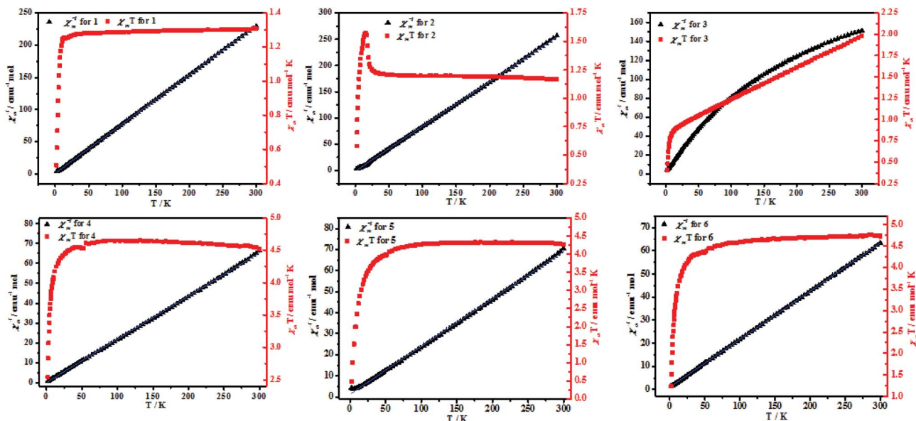
Fig. 7 Temperature-dependent magnetic susceptibilities of 4–6 in the temperature range of 2–300 K under an applied magnetic field of 1000 O.
