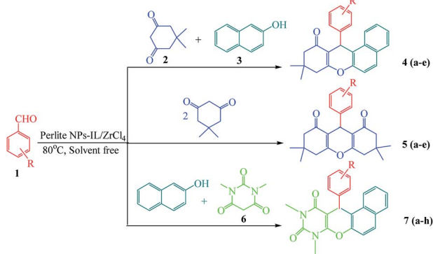
Scheme 1 Solvent free one-pot synthesis of three types of xanthenes derivatives in the presence of perlite NPs@IL/ZrCl 4 .
