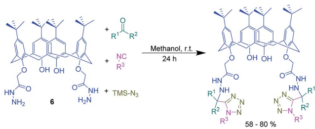
Scheme 11 Ugi-azide-4-component reaction of calixarene dihydrazide 6 .
