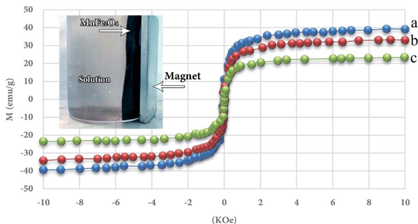
Fig. 4 Magnetic curves for MnFe 2 O 4 (a), MnFe 2 O 4 -TiO 2 (b) and -MnFe 2 O 4 -TiO 2 UIO-66 (c).
