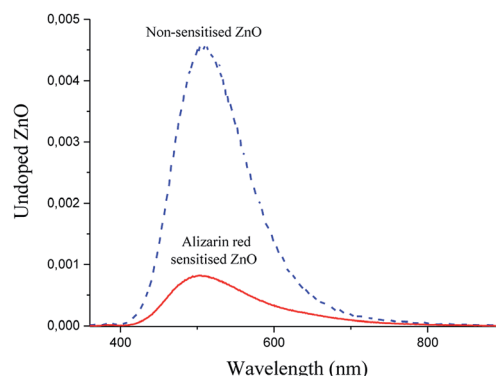
Fig. 5 Photoluminescence spectra of alizarin red sensitised zinc oxide (solid red line) and non-sensitised ZnO (dashed blue). The lowered peak intensity of alizarin red sensitised zinc oxide (solid red line) has indicated fewer electron–hole recombinations between the conduction band and intrinsic defect site of zinc oxide.
