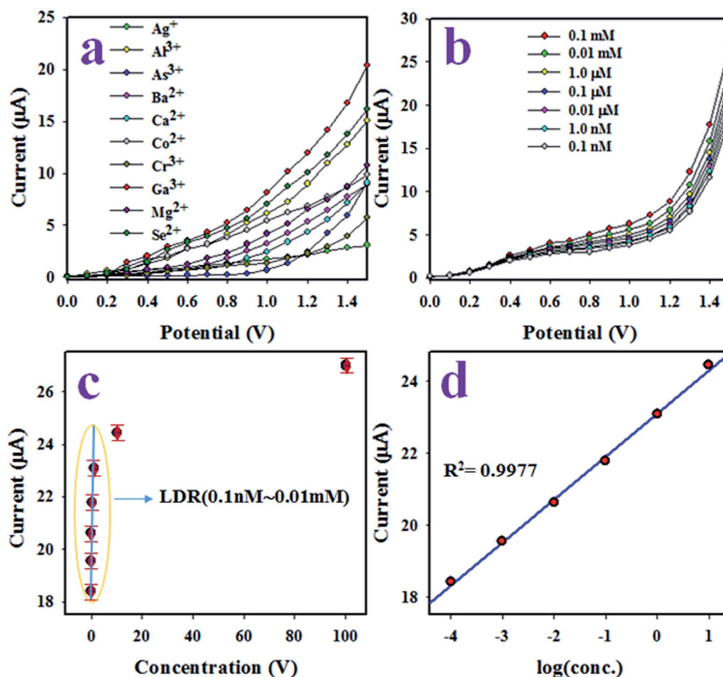
Fig. 12 The electrochemical ( I - V ) characterization of sensor based on \text{P}(\text{Py-co-OT})/\text{CF}/\text{R}(\text{GO-OXSWCNTs}) \text{ NCs}/\text{binder}/\text{GCE} . (a) The identification of selectivity, (b) the variation of I - V responses of \text{Ga}^{3+} ion with a variation of concentration from lower to higher, (c) the calibration of \text{Ga}^{3+} ion sensor and (d) \log(\text{conc.}) vs. current.
