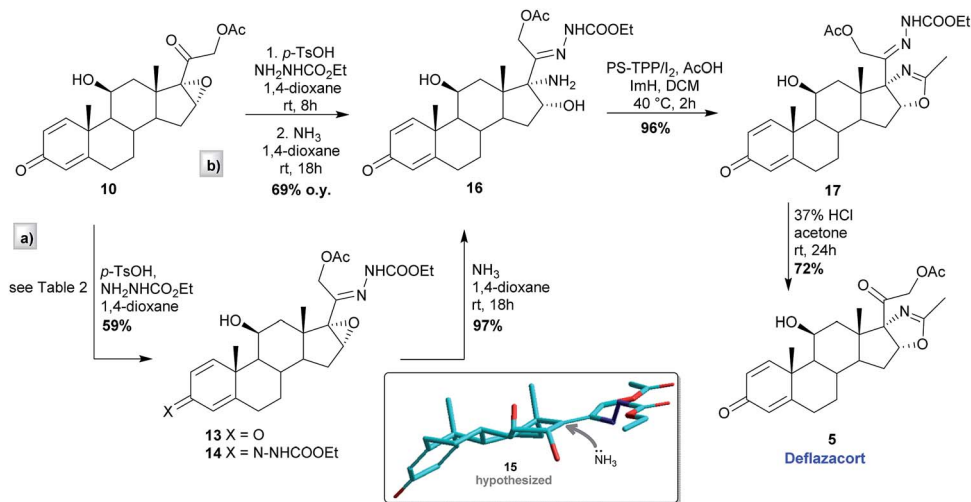
Scheme 2 Synthetic steps to deflazacort from epoxide 10.
