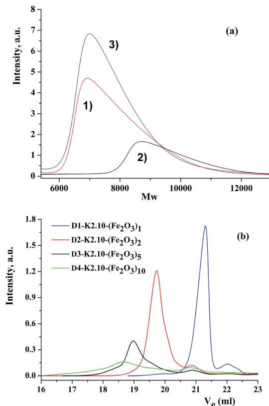
Fig. 3 (a) GPC-chromatograms of the complex, nanocomposite and ligand; (b) GPC-chromatograms of nanocomposites from the first to the fourth generation. (1) Free metal dendrimer; (2) dendritic complex and (3) nanocomposite D1-K2.10- (\text{Fe}_2\text{O}_3)_1 .
