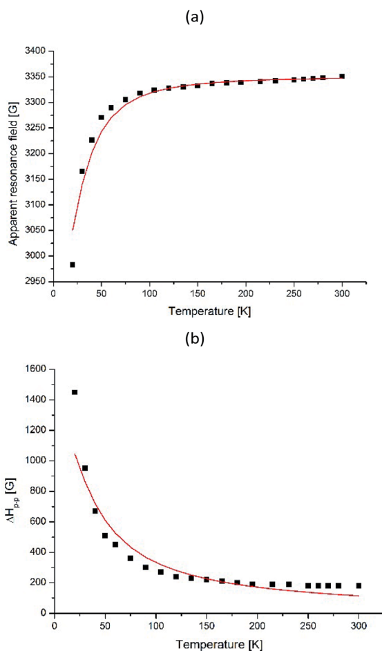
Fig. 14 Temperature dependences of H_{\text{res}} (a) and \Delta H_{\text{p-p}} (b) for I-type Fe(III) centers for \gamma -Fe 2 O 3 NPs in dendrimers. The solid line shows the theoretical dependence simulated by BK theory given by eqn (3) and (5) for (a) and (b), respectively.
