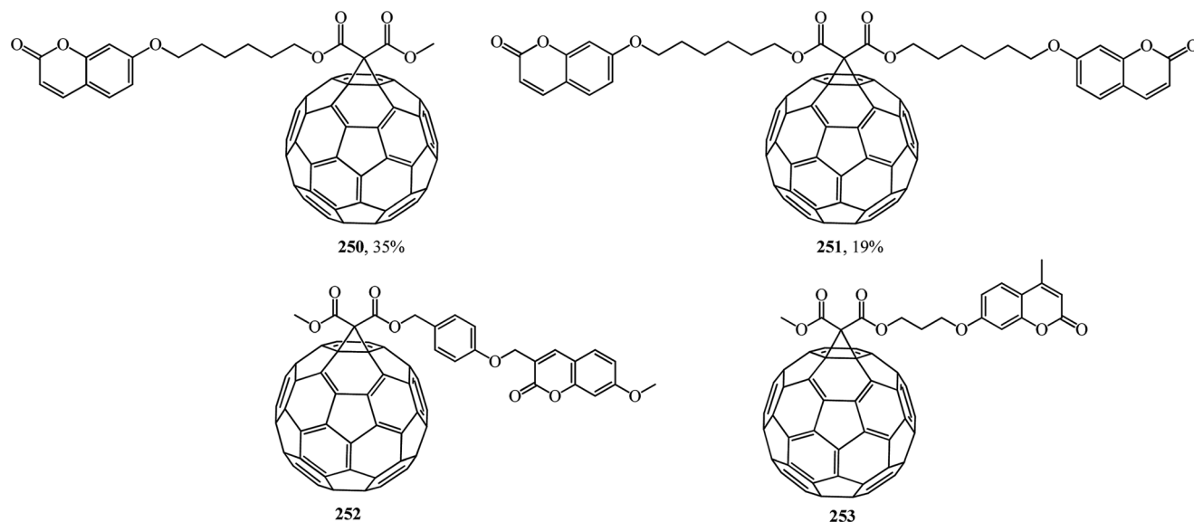
Fig. 14 Fullerene-coumarin diads 250–253.
