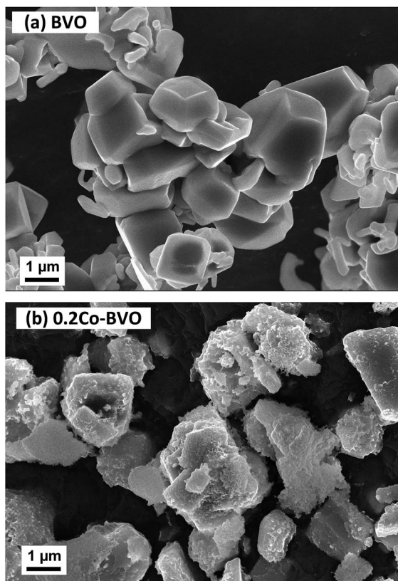
Fig. 3 SEM images of the (a) BVO and (b) 0.2Co-BVO samples.
