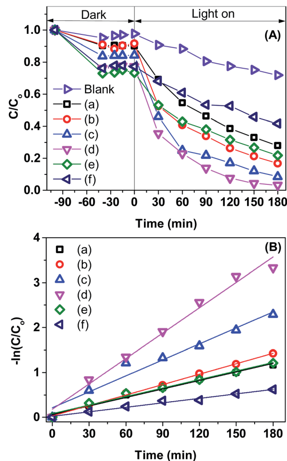
Fig. 8 Photocatalytic degradation of MB over BiVO 4 samples (A): BiVO 4 (a), 0.05Co-BVO (b), 0.1Co-BV (c), 0.2Co-BV (d), 0.3Co-BV4 (e), and 0.5Co-BV (f) and plots of \ln(C_0/C) versus irradiation time representing the fit using a pseudo-first-order reaction rate (B).
