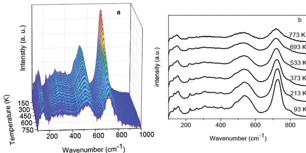
Fig. 4 (a) Full temperature-dependent Raman spectra of the Zn_{1.8}Co_{0.2}TiO_4 crystal in the range from 93 to 773 K. (b) Selected temperature-dependent Raman spectra.
