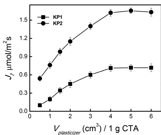
Fig. 9 The effect of o -NPPE plasticizer on the Ag(I) transport through PIM. Source phase: 5.0 × 10 -4 M AgNO 3 , pH = 4.0; membrane: 25.0 mg CTA; 0.10 M KP1 and KP2, receiving phase: 0.10 M Na 2 S 2 O 3 .
