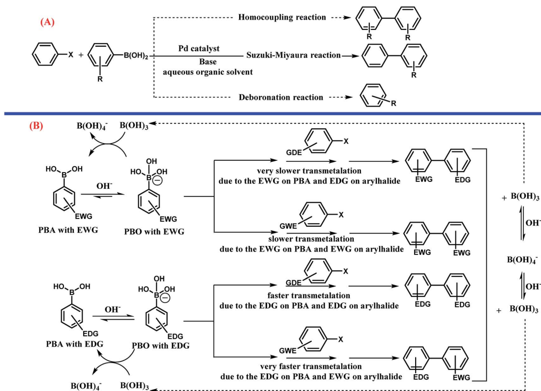
Scheme 7 (A) The competing reactions (homocoupling and deboronation) with the Suzuki–Miyaura cross coupling reaction (—: competition reaction, - - - : main reaction). (B) The effect of electron-withdrawing group (EWG) and electron-donating group (EDG) on phenylboronic acid (PBA), phenylborate (PBO), and aryl halides on the rate of the Suzuki–Miyaura cross coupling reaction.
