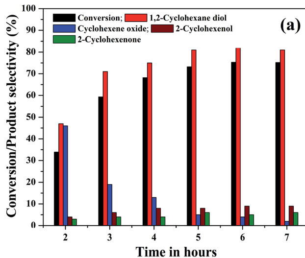
Fig. 10 (a) Effect of reaction time on the cyclohexene conversion and products selectivity (cyclohexene: 2 mmol, \text{H}_2\text{O}_2 : 10 mmol, acetonitrile: 5 ml, catalyst: 5% rGO/Fe 3 O 4 nanocomposite, catalyst dosage: 0.05 g, temperature: 70 °C, atmospheric pressure).
