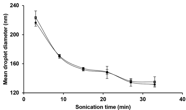
Fig. 4 Effects of sonication time and storage (day 1 ● and day 30 □) on the mean droplet diameter of nanoemulsions (10 wt% sunflower oil, 2 wt% saponin).
