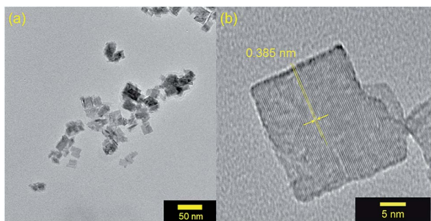
Fig. 8 (a) TEM images of MW- \text{WO}_3 particles after photocatalysis on benzyl alcohol. (b) High resolution TEM image of a \text{WO}_3 nanoplatelet after photocatalysis.
