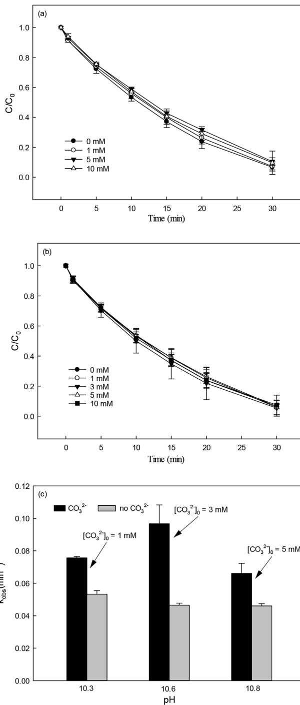
Fig. 6 Effect of \text{NO}_3^- (a), \text{SO}_4^{2-} (b) and \text{CO}_3^{2-} (c) on DCF degradation in HAP system. Experimental conditions: [\text{DCF}]_0 = 1 \mu\text{M} , [\text{PS}]_0 = 50 \mu\text{M} , 5 mM phosphate buffer at pH = 6.2 for \text{NO}_3^- and \text{SO}_4^{2-} groups, no buffer for \text{CO}_3^{2-} group.
