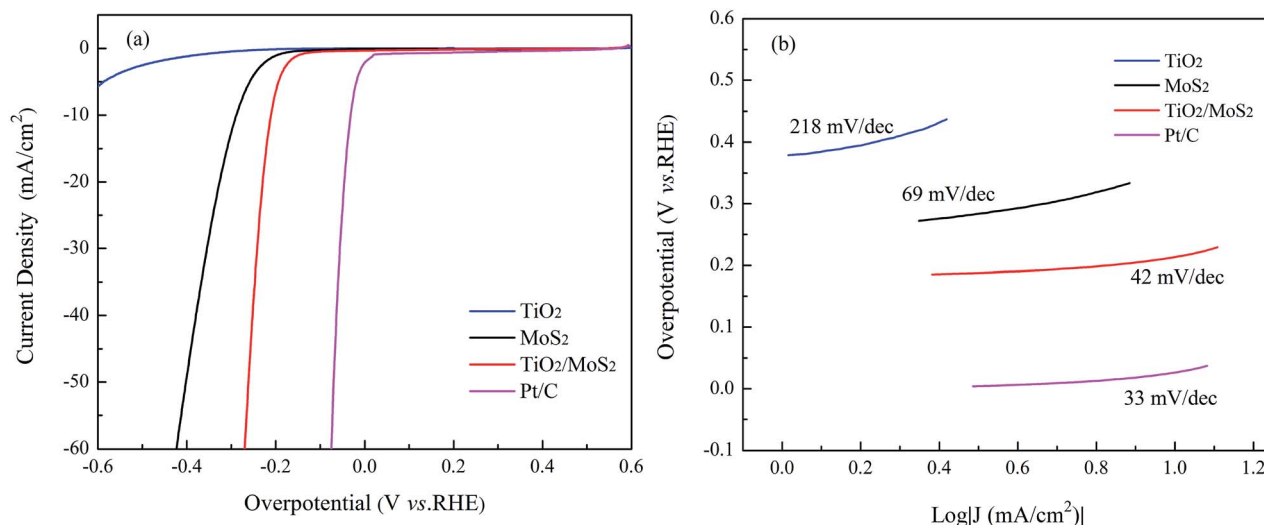
Fig. 4 (a) Polarization curves and (b) the corresponding Tafel plots of TiO 2 , MoS 2 -NTs and TiO 2 /MoS 2 -NTs in 0.5 M H 2 SO 4 solution.
