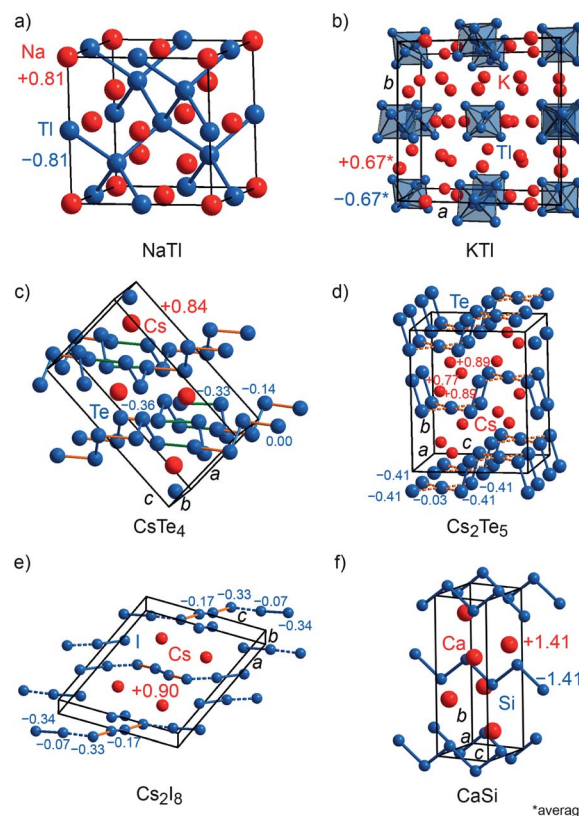
Fig. 3 (a) Representations of the crystal structures of sodium thallide, (b) potassium thallide, (c) CsTe_4 , (d) Cs_2Te_5 , (e) Cs_2I_8 and (f) calcium silicide. Mulliken charges are shown. To distinguish bonds within the anions from those contacts between the anions, the contacts within the anions have been highlighted using different colors.
