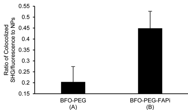
Fig. 4 Association of BFO-PEG NPs and BFO-PEG-FAPi NPs to hrFAP quantified by multiphoton multispectral microscopy. HrFAP (100 ng) was incubated for 2 h at 37 °C with BFO-PEG NPs (100 \mu\text{g mL}^{-1} ) (A) or BFO-PEG-FAPi NPs (100 \mu\text{g mL}^{-1} ) (B) in the presence of Human Fibroblast Activation Protein alpha/FAP Alexa Fluor® 594-conjugated Antibody (dilution 1 : 5). SH and fluorescence signals were epi-collected upon focused excitation at 840 nm. The ratio of the area of conjugates emitting in both SH and fluorescence channels to the area of SH emitting structures was averaged from four distinct regions of each sample (635 \times 635 \mu\text{m} ). Error bars represent standard deviation from n = 4 calculations.
