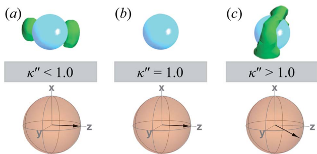
Fig. 7 A visual summary of topological defects for single-colloid systems in a N_D solvent: (a) boojums form with planar anchoring [ i.e. , \kappa'' < 1 ], (b) no discernible defects arise when no anchoring type is energetically preferred [ i.e. , \kappa'' = 1 ], and (c) Saturn rings emerge with homeotropic anchoring [ i.e. , \kappa'' > 1 ]. The average orientation of the director is shown below each rendition, indicated by the sphere-referenced coordinate system.
