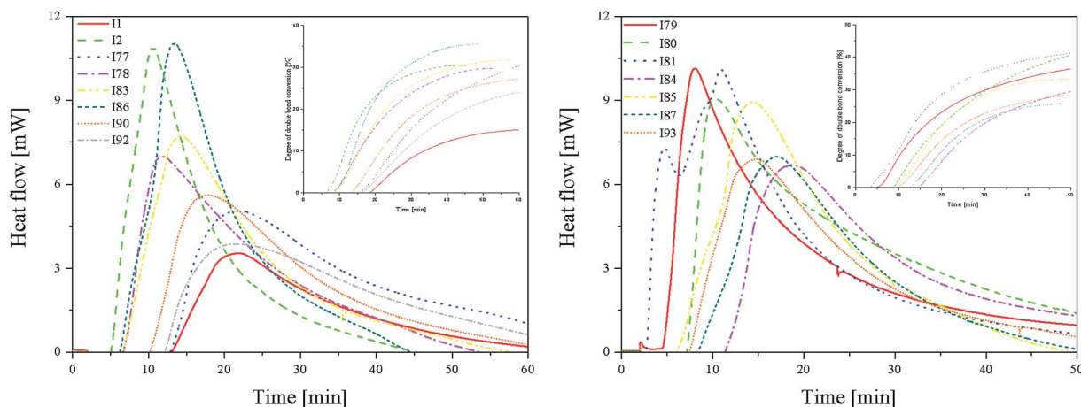
Fig. 4 The kinetic curves recorded during the radical polymerization of TMPTA initiated by 2-( p - N,N -dimethylaminostyryl)benzoxazole in the presence of coin initiators (L): with an activating substituent in the p -position and (R): with a deactivating substituent in the p -position. Inset: time-conversion curves of polymerization reaction in the presence of different radical sources (marked in figure).
