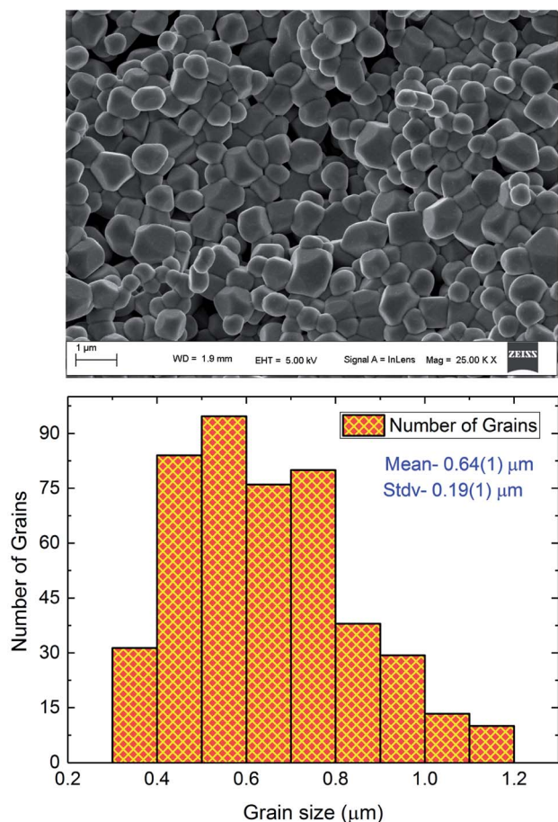
Fig. 2 The SEM micrograph of Pr 0.8 Na 0.2 MnO 3 and histogram of grain size distribution.
