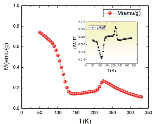
Fig. 3 Temperature dependence of the magnetization at 0.05 T for Pr 0.8 Na 0.2 MnO 3 sample. The inset is the dM/dT curve.
