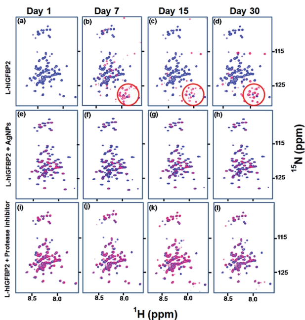
Fig. 8 Stability studies of L-hIGFBP2: (a–d) shows the overlay of 2D [ ^{15}\text{N} , ^1\text{H} ] HSQC spectra of free L-hIGFBP2 (blue) with that of the protein sample at different time intervals (red). The encircled part shows the degradation peaks appearing with time; (e–h) overlay of 2D [ ^{15}\text{N} , ^1\text{H} ] HSQC spectra of free L-hIGFBP2 (blue) with that of the protein in presence of 30 nM AgNPs (red) (see also Fig. 4); (i–l) show the overlay of the spectra of free L-hIGFBP2 (blue) with that of the protein in presence of the protease inhibitor cocktail (red) at different intervals of time (indicated on the top).
