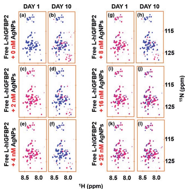
Fig. 9 Overlay of 2D [ ^{15}\text{N} , ^1\text{H} ] HSQC spectra of free L-hIGFBP2 (blue) with that of the protein samples at different concentration of AgNPs (red) on Day 1 and Day 10. The different concentrations of AgNP used in (a)–(l) are indicated on the left of each set.
