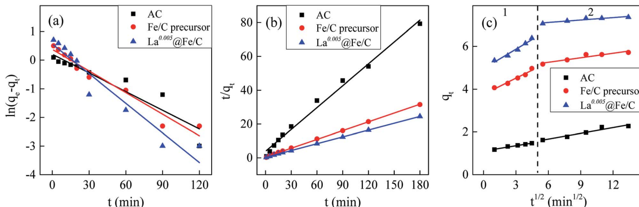
Fig. 8 Kinetic modeling of: (a) pseudo-first-order model, (b) pseudo-second-order model, and (c) intra-particle diffusion model for phosphate adsorption on the adsorbents.
