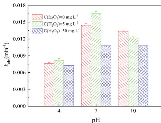
Fig. 5 Effect of solution pH on the pseudo-first-order reaction rate constants ( k_{\text{obs}} ) of ATZ during UV irradiation treatment under different \text{H}_2\text{O}_2 doses. Raw ATZ solution: 5 \text{ mg L}^{-1} .
