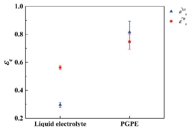
Fig. 7 Effective charges for Li (blue triangles) and TFSI (red circles) at 20 °C measured by 7 Li and 19 F NMR respectively. Errors are calculated by error propagation.
