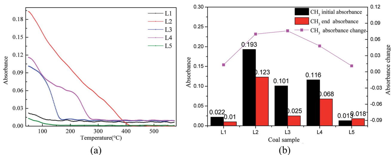
Fig. 8 Changes in the -CH_3 bonds at 2975\text{ cm}^{-1} during coal spontaneous combustion: (a) the amounts of the functional group at each temperature; (b) the degrees of participation of the functional group.
