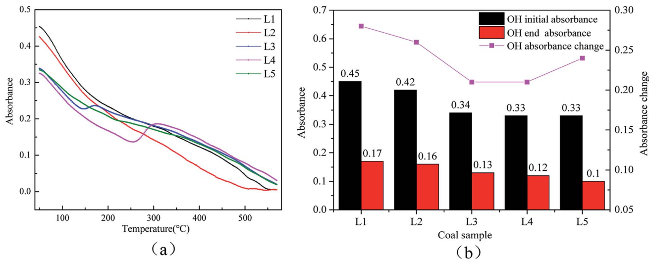
Fig. 7 Changes in the -OH bond at 3485\text{ cm}^{-1} during coal spontaneous combustion: (a) the amounts of the functional group at each temperature; (b) the degrees of participation of the functional group.
