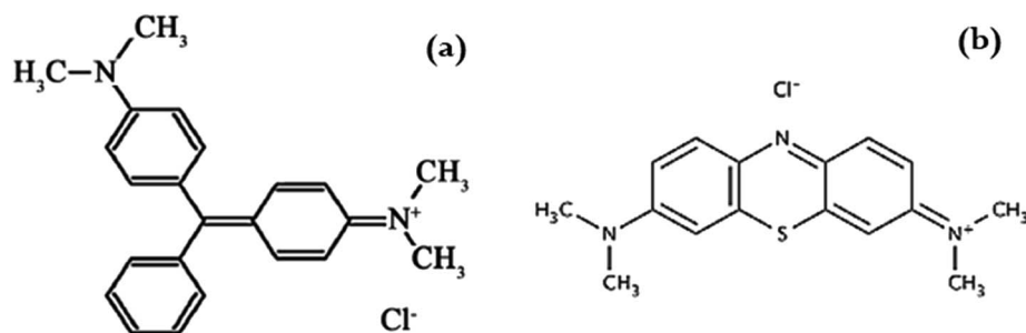
Fig. 1 Structures of (a) malachite green and (b) methylene blue.
