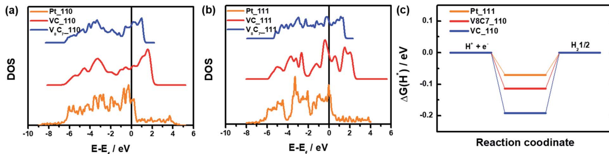
Fig. 6 (a) and (b) are calculated DOS of VC, V 8 C 7 and Pt on their (110) and (111) surfaces. Curves are shifted vertically for clarity. (c) |\Delta G(\text{H}^*)| values of VC, V 8 C 7 and Pt.
