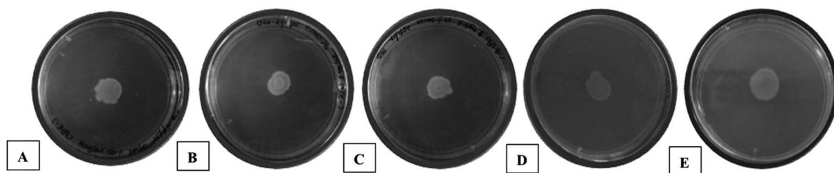
Fig. 5 Inhibition of swarming activity of P. aeruginosa by compound 7 in dose-dependent manner – (A) 4 \text{ mg mL}^{-1} ( 16.5 \pm 1 \text{ mm} ), (B) 6 \text{ mg mL}^{-1} ( 15 \pm 1.3 \text{ mm} ), (C) 8 \text{ mg mL}^{-1} ( 14 \pm 1 \text{ mm} ) along with (D) negative control (50% DMSO) ( 20.5 \pm 1.2 \text{ mm} ) and (E) untreated P. aeruginosa ( 21.5 \pm 1 \text{ mm} ).
