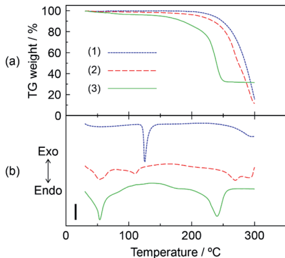
Fig. 1 TG (a) and DTA (b) curves of (1) DOT material, (2) DOT-40 mol% MDP composite material, and (3) MDP material. These measurements were done at the heating rate of 10 °C min -1 under flowing dry-nitrogen. The TG-DTA measurements were normalized at 1 mg. Scale bar in (b) indicates 10 μV mg -1 . Triplicate experiments gave similar results.
