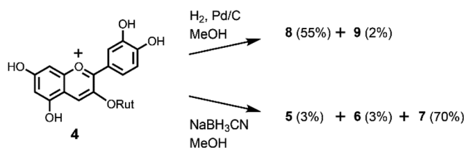
Scheme 4 Reduction of 4 .
