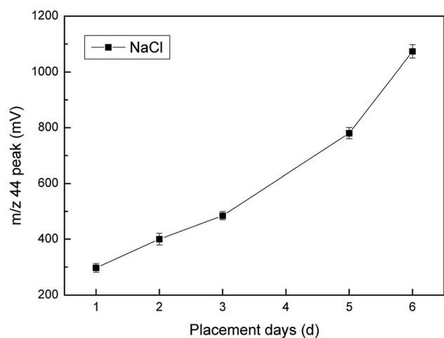
Fig. 5 Correlation between the NaCl placement days and its m/z 44 peak amplitude.
