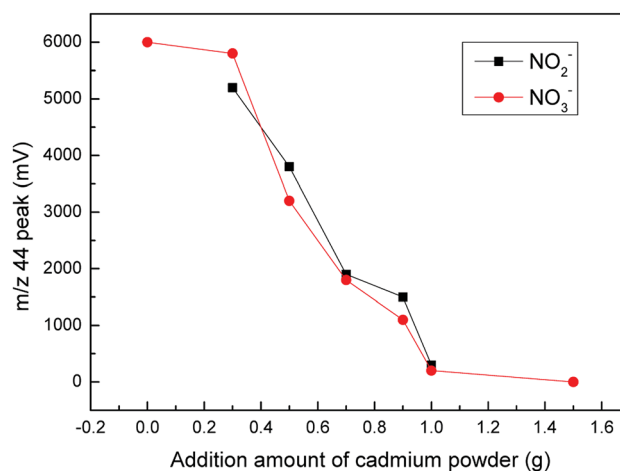
Fig. 6 Relationship between the m/z 44 peak amplitudes for the NO_3^- , NO_2^- and Cd powder addition.
