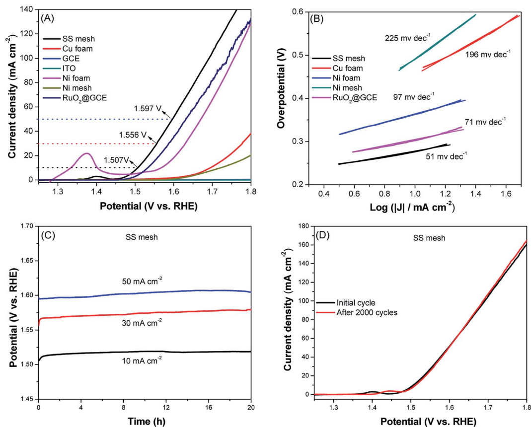
Fig. 5 (A) The LSV curves measured at 2 \text{ mV s}^{-1} in 1 \text{ M KOH} solution for OER and (B) the corresponding Tafel slopes; (C) chronopotentiometric curves at different current density; (D) LSV curves obtained with SS mesh before and after 2000 cycles of an accelerated stability test.
