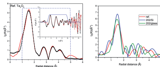
Fig. 2 EXAFS analysis of the L_{3} Ta edge in radial distance of the coordination spheres up to 5.0 Å in reference Ta_2O_5 powder. The measured spectra – red, fit – dotted black, fitting window – dashed blue line; inset: data and fit in wavenumber k (left). Comparison of the Fourier transform spectra of the reference and 202 nm films (right).
