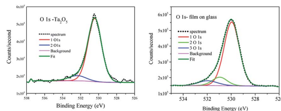
Fig. 5 XPS of O 1s for reference \text{Ta}_2\text{O}_5 powder (left) and for 202 nm on glass amorphous film (right).
