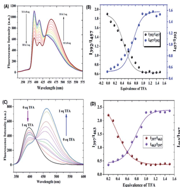
Fig. 4 (A) Emission spectra of the compound 2a ( 2 \times 10^{-5} M) in chloroform solvent over the addition of TFA ( \lambda_{\text{ex}} = 267 nm). (B) Sigmoidal fitting of fluorescence intensity ratio I_{392}/I_{457} vs. equivalence of TFA for compound 2a . (C) Emission spectra of the compound 2b ( 2 \times 10^{-5} M) in chloroform solvent over the addition of TFA ( \lambda_{\text{ex}} = 267 nm). (D) Sigmoidal fitting of fluorescence intensity ratio I_{397}/I_{463} vs. equivalence of TFA for compound 2a .
