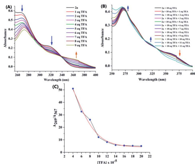
Fig. 3 (A) The absorption spectra of the compound 2a ( 2 \times 10^{-5} M) in chloroform solvent over the addition of TFA. (B) The absorption spectra of the compound 2b with TFA over the addition of TEA. (C) The plot of absorption intensity ratio ( A_{269}/A_{367} ) vs. the concentration of TFA.
