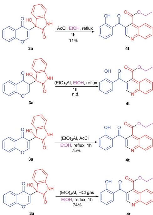
Scheme 2 Control experiments.
