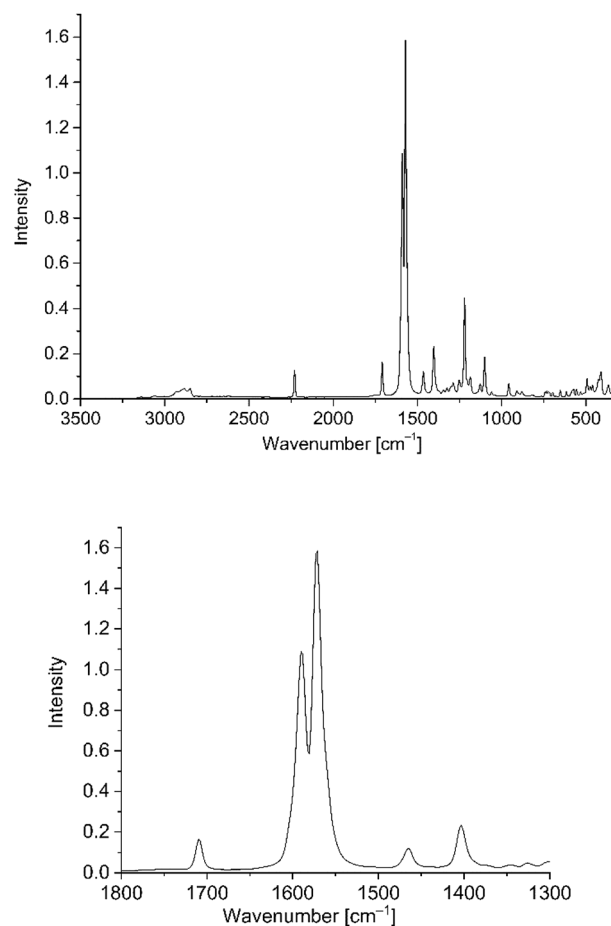
Fig. 4 Solid-state Raman spectrum of PD 1 (top) as overview from 3500 to 500 \text{ cm}^{-1} and (bottom) with the relevant C=C stretching region from 1800 to 1300 \text{ cm}^{-1} which was used for the subsequent SERS studies. It is important, that the signal at 1600 \text{ cm}^{-1} does not interfere with the solvent signals from the water/acetone mixture (Fig. S7 in ESI†).
