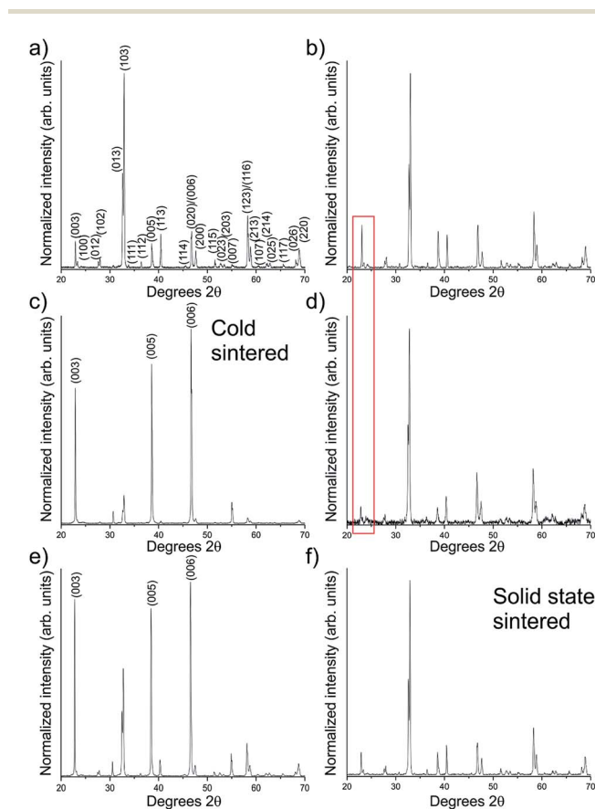
Fig. 3 X-ray diffraction patterns for (a) the as-prepared YBCO powder, showing normal relative intensities. (b) Shows the same powder ground with water in preparation for cold sintering. Some overexpression of the (00 l ) faces is observed. (c) Pattern obtained from the top surface of a cold sintered ceramic showing significant (00 l ) plane overexpression, in contrast to the inner surface of the same ceramic in (d) which shows a corresponding under-expression of the (00 l ) planes. Red box highlights the difference in relative intensities of the (003) reflection in the powder vs. the internal surface of the cold sintered pellet, indicating a relative decrease. The (00 l ) overexpression is also observed in (e), which is a sample uniaxially pressed at room temperature ready for standard solid state sintering, which also shows some overexpression in the c -direction, in contrast to the same sample after sintering at 1000 °C in (f) which has returned to its isotropically axed state.
